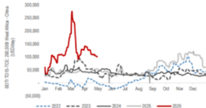
Figure 1: West Africa-China VLCC TCE (TD15): Declining to US$100k/day as Atlantic routes normalize
